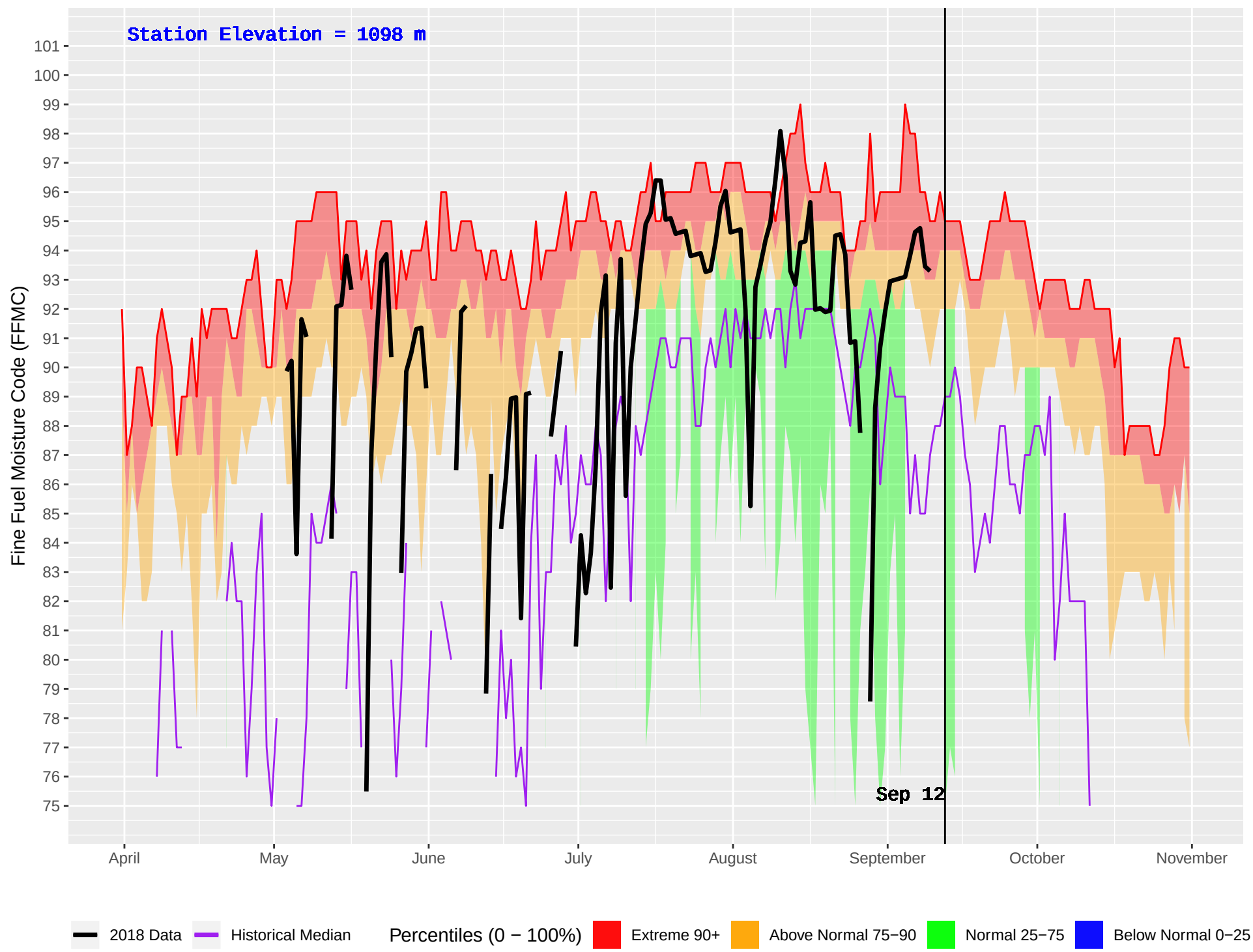
GOATFELL (401) : Historical (1986–2016) and Current (2018) Daily Fine Fuel Moisture Code (FFMC)
