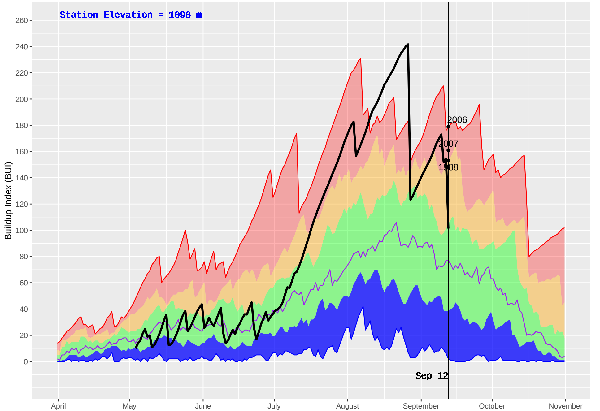
GOATFELL (401) : Historical (1986–2016) and Current (2018) Daily Buildup Index (BUI)
